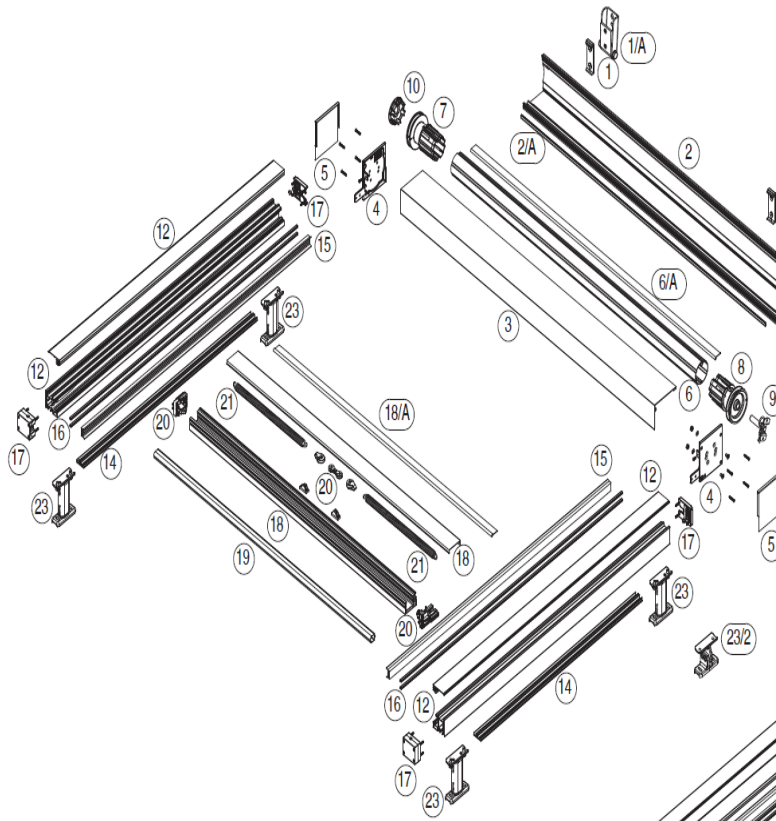
vista posteriore - rear view
